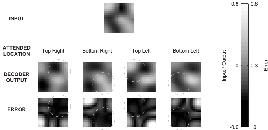
Fig. 2. Reconstruction example for a single input pattern and four different attentional states as indicated by the dashed circles. The error is calculated as the absolute intensity difference between input and output.
